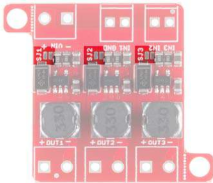
Solder Jumpers
