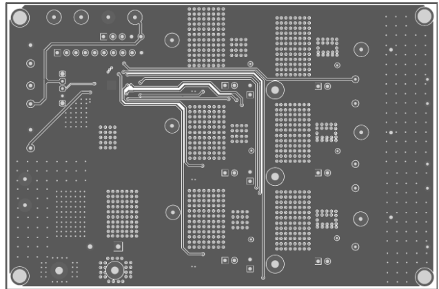
Figure 4: Inner 2 Layer
