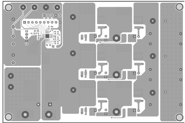
Figure 2: Top Layer
