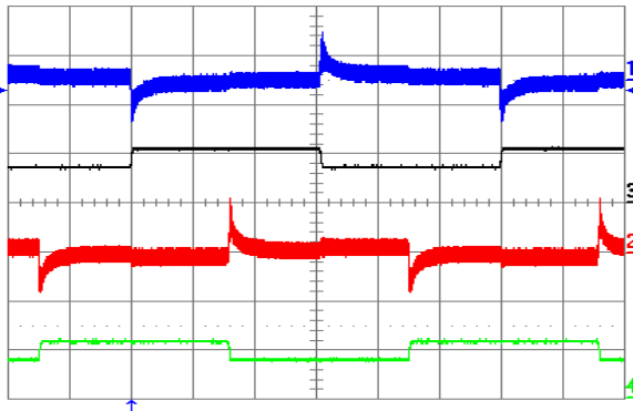
Figure 23. Output voltage response to both Iout1 and Iout2 (out of phase) load current step-change of 3.75 A (50%-75%-50%) at Vin = 48 V. Ch1 = Vout1 (50 mV/div), Ch2 = Vout2 (50 mV/div), Ch3 = Iout1 (10 A/div.), Ch4 = Iout2 (10 A/div.). Current slew rate: 0.1 A/μs, Co = 10 μF tantalum + 1 μF ceramic. Time scale: 1 ms/div.
