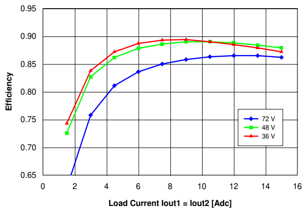
Figure 16. Efficiency vs. balanced load current ( I_{out1} = I_{out2} ) and input voltage for converter mounted horizontally with air flowing from pin 3 to pin 4 at a rate of 300 LFM (1.5 m/s) and T_a = 25 °C.
