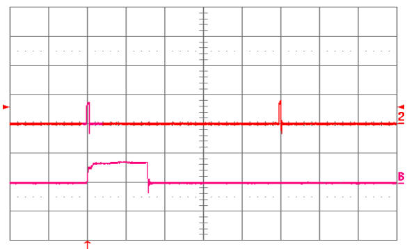
Figure 28. Load current Iout2 into a 10 mΩ short circuit on Vout2 during restart, with Vout1 open (no load), at Vin = 48 V. Ch2 = Iout2 (20 A/div, 20 ms/div). ChB = Iout2 (20 A/div, 1 ms/div) is an expansion of the on-time portion of Iout2.
