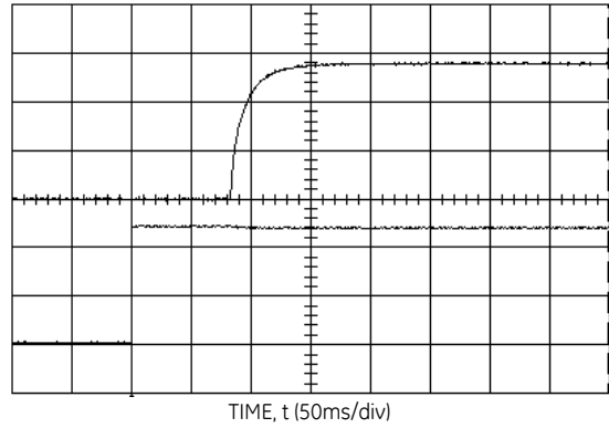
Figure 5. Typical Start-Up Using from V IN , positive logic version shown; C o,ext = 470µF.
