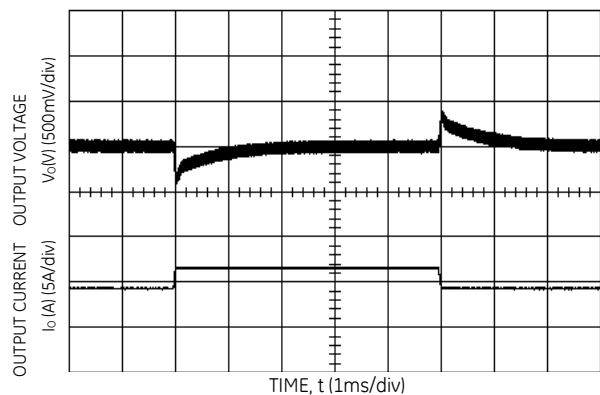
Figure 6. Transient Response to Dynamic Load Change from 50% to 75% to 50% of Full Load at Room Temperature and 48 Vdc Input; 0.1A/uS
