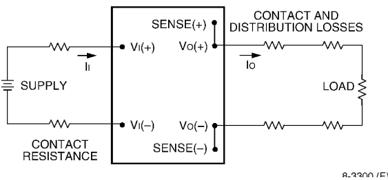
Figure 9. Output Voltage and Efficiency Test Setup.
