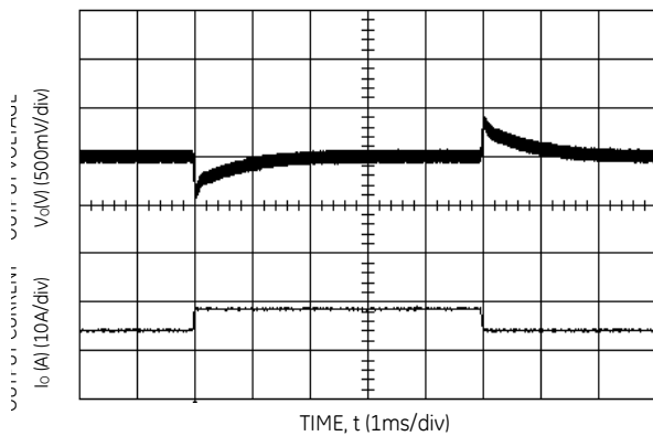
Figure 3. Transient Response to Dynamic Load Change from 25% to 50% to 25% of Full Load at Room Temperature and 48 Vdc Input; 0.1A/uS
