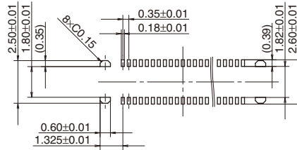
Recommended metal mask pattern Metal mask thickness: When 100μm (Terminal opening ratio: 70%) (Metal-part opening ratio: 46%)
