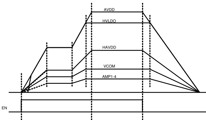
Figure 48. Timing Chart 2
