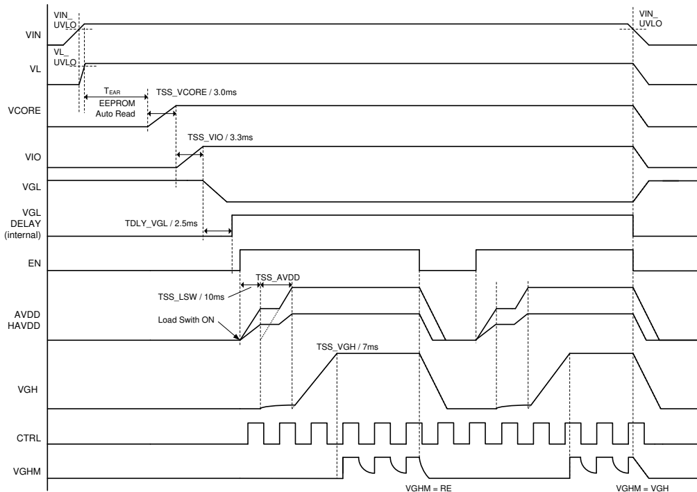
Figure 47. Timing Chart
