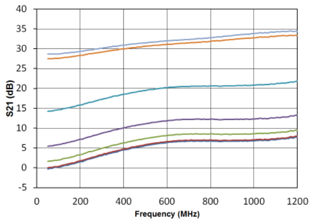
Receiver Gain
