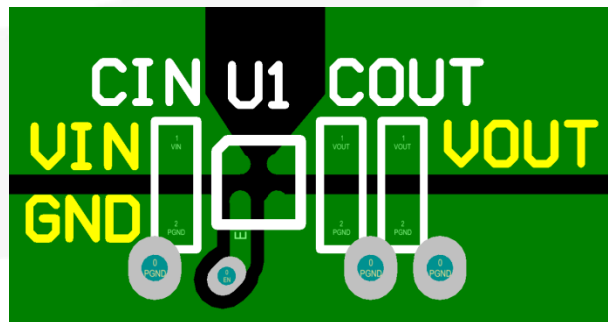
Figure 18. Recommended Layout
