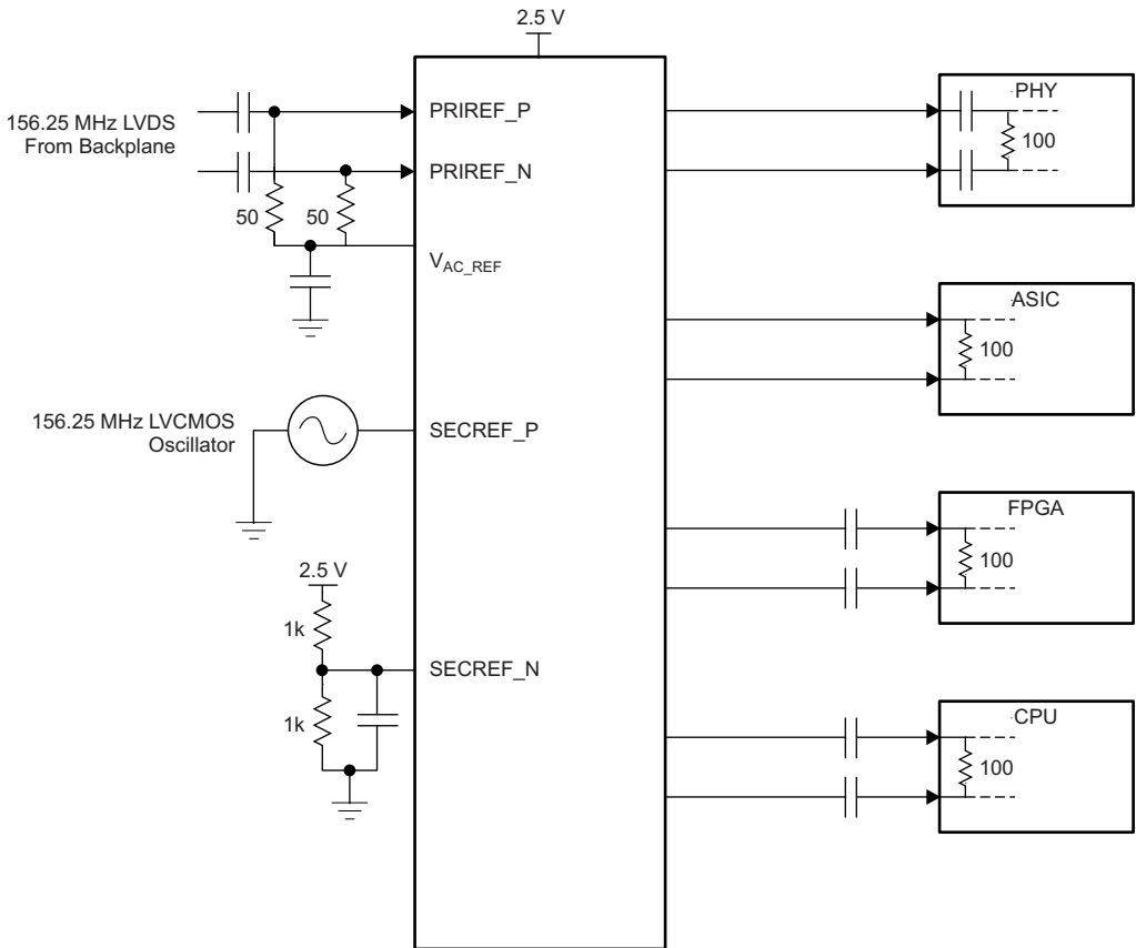
Figure 14. Fan-Out Buffer for Line Card Application
