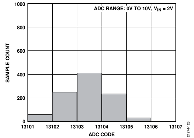
Figure 30. ADC Noise Histogram with ODR = 4 kSPS
