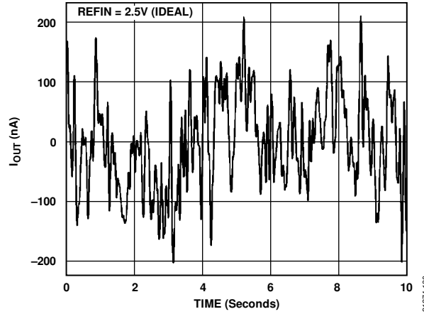
Figure 23. Peak-to-Peak Noise (0.1 Hz to 10 Hz Bandwidth)
