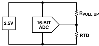
Figure 40. RTD Bias Circuit
