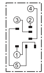
Internal Connections (Top View)
