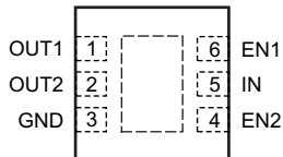
DPQ Package 6-Pin X2SON Top View
