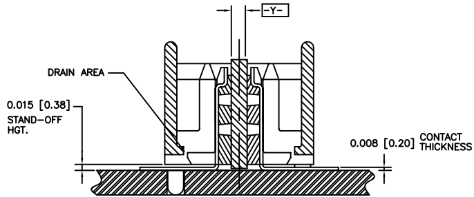
SECTION M-M ROTATED COUNTERCLOCKWISE 90° SCALE 2:1
