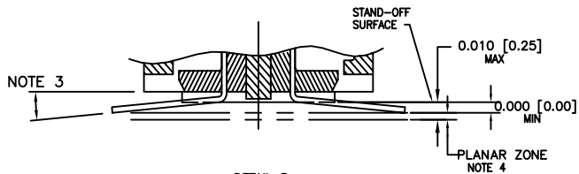
DETAIL B SCALE 3:1
