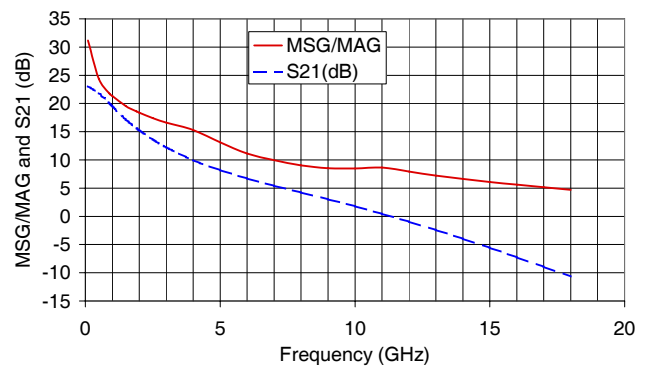
MAXIMUM STABLE GAIN (MSG)/MAXIMUM AVAILABLE GAIN (MAG) vs. FREQUENCY V_{DS}=3V & I_{DS}=10\text{ mA}
