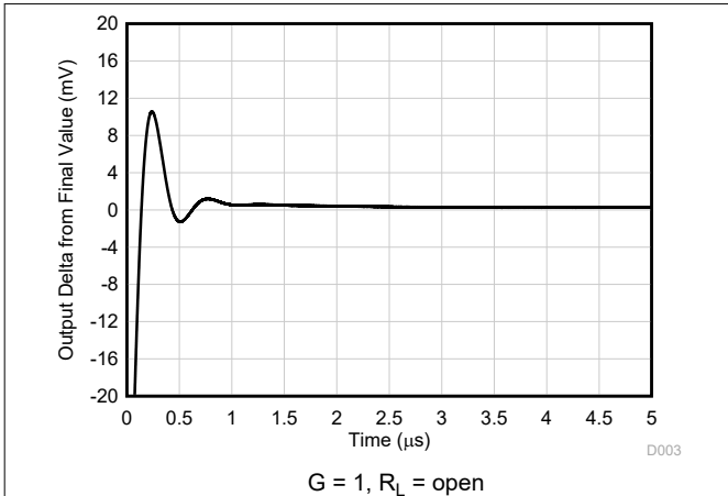
Figure 6-31. Large-Signal Step Response (Rising)
