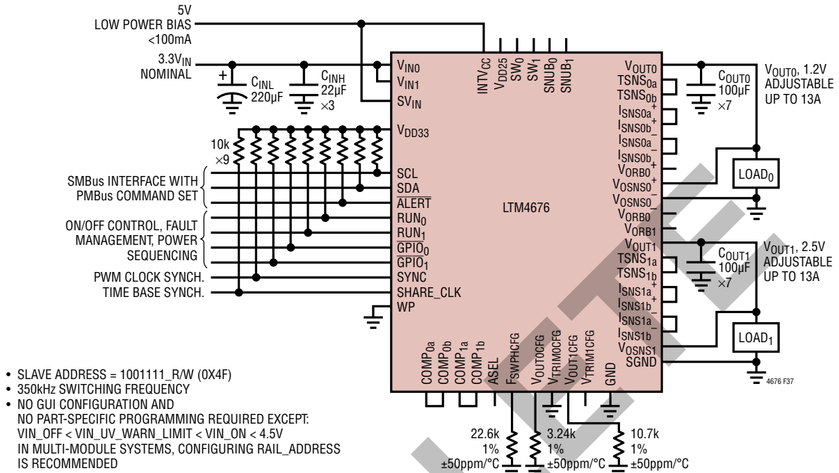
Figure 37. 1.2V and 2.5V Outputs Generated from 3.3V Power Input and Providing I 2 C/SMBus/PMBus Serial Interface
