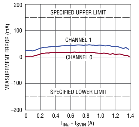
MFR_READ_IIN n (Input Current Readback) Error vs (I_{\text{VIN}n} + I_{\text{SVIN}}) , \text{MFR\_PWM\_MODE}_n[1:0] = 10_{\text{b}} , I_{\text{OUT}n} Swept from 0\text{A} to 13\text{A} , One Channel at a Time, \text{RUN}_{1-n} = 0\text{V}
