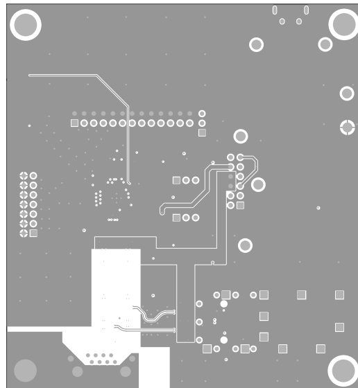
Figure 25. Signal Layer 4
