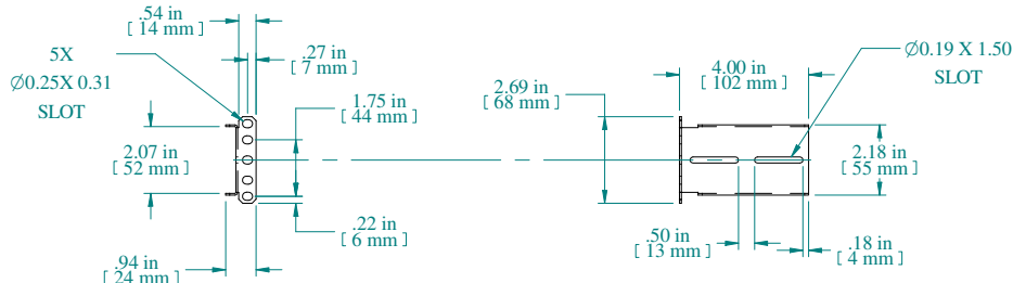
SLIDE RAIL MOUNT BRACKETS
