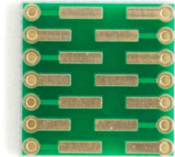
2D Bottom View (Pins Unassembled)
