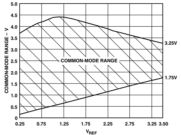
Figure 8. Input Common-Mode Range vs. V_{REF} ( V_{DD} = 5 V and V_{REF} (\text{Max}) = 3.5 V)
