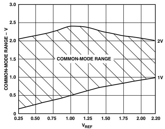
Figure 9. Input Common-Mode Range vs. V_{REF} ( V_{DD} = 3 V and V_{REF} (\text{Max}) = 2.2 V)
