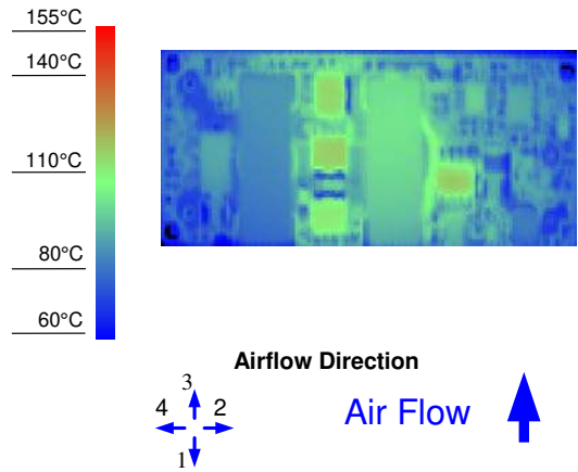
Figure 8. Thermal Image for Airflow Direction 3 (40A output, 55°C ambient, 200 LFM, typical Vin, open frame unit)
