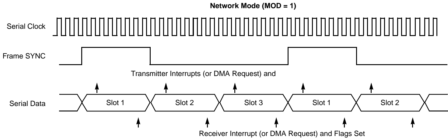
Figure 7-8. CRB MOD Bit Operation
