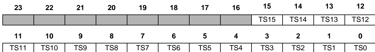
—Reserved bit; read as 0; write to 0 0 for future compatibility. (ESSI0 X:$FFFFB4, ESSI1 X:$FFFA4)
