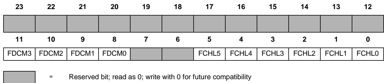
Figure 10-14. Decimation/Channel Count Register (FDCH)
