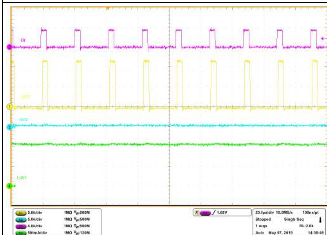
Chan. 1 = IOUT Chan. 2 = OUT2 Chan. 3 = EN/IN1 Chan. 4 = IOUT
