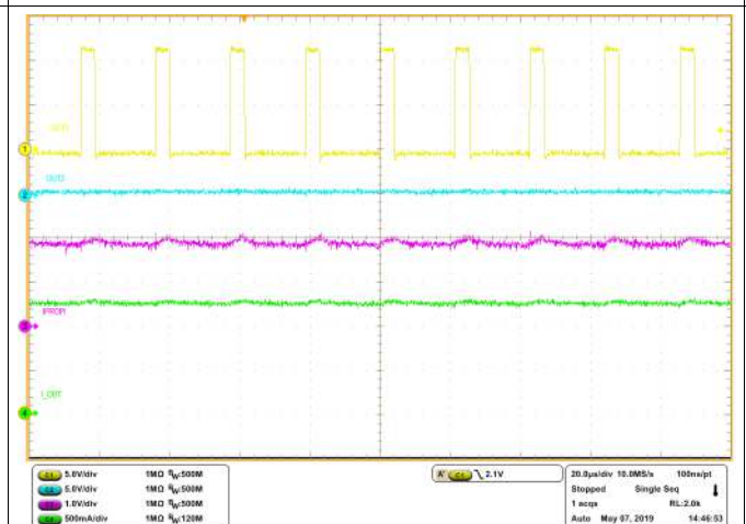
Chan. 1 = IOUT Chan. 2 = OUT2 Chan. 3 = IPROPI Chan. 4 = IOUT
