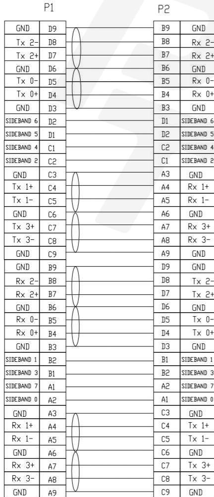
WIRING DIAGRAM
