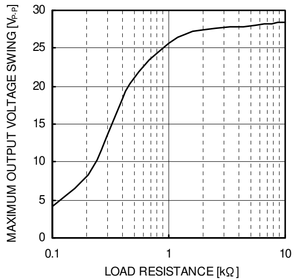
Figure 5. Maximum Output Voltage Swing - Load Resistance (VCC/VEE=±15V, Ta=25°C)
