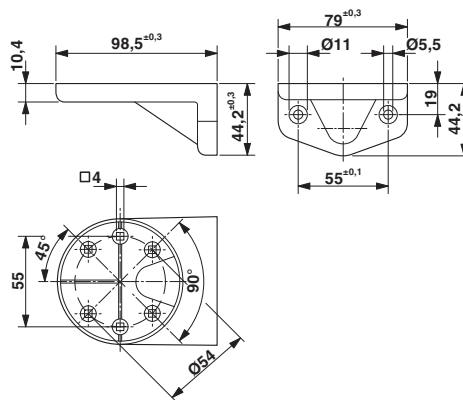
Dimensioned drawing
