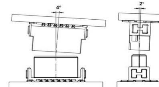
Admissible inclination
