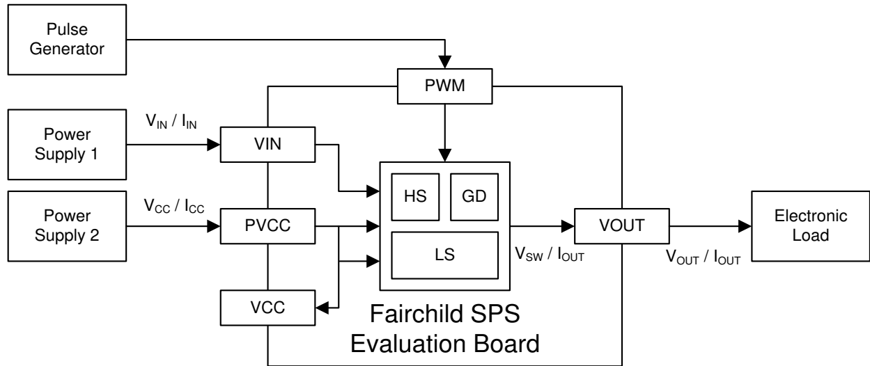
Figure 29. Power Loss and Efficiency Measurement Diagram
