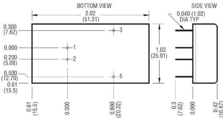
Figure 2. Mechanical Dimensions
