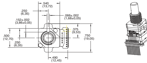
SERIES 62HR WITH .050 CENTER TERMINAL PINS
