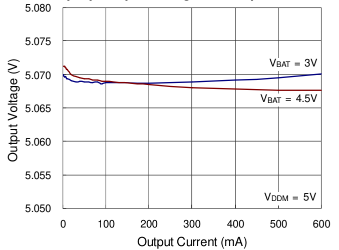
CH1 Step-Up Output Voltage vs. Output Current
