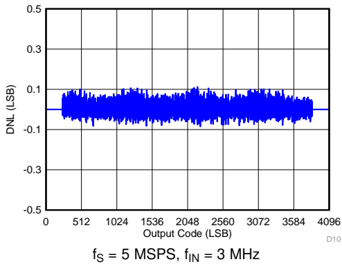
Figure 126. Differential Non-linearity at 5-MSPS Sampling Speed
