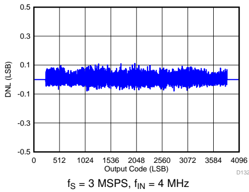
Figure 124. Differential Nonlinearity at 3-MSPS Sampling Speed
