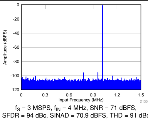
Figure 114. FFT for 3-MSPS Sampling Speed
