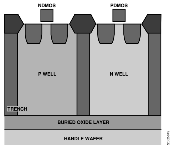
Figure 45. Trench Isolation
