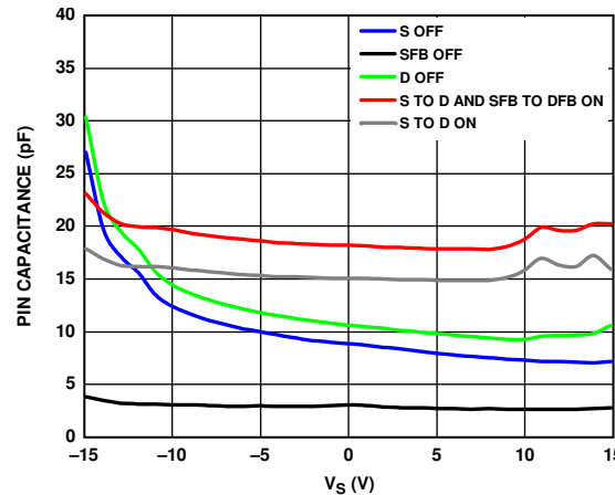
Figure 25. Pin Capacitance vs. V_S
