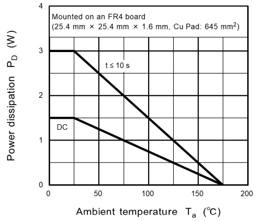
Fig. 8.14 P_D - T_a
