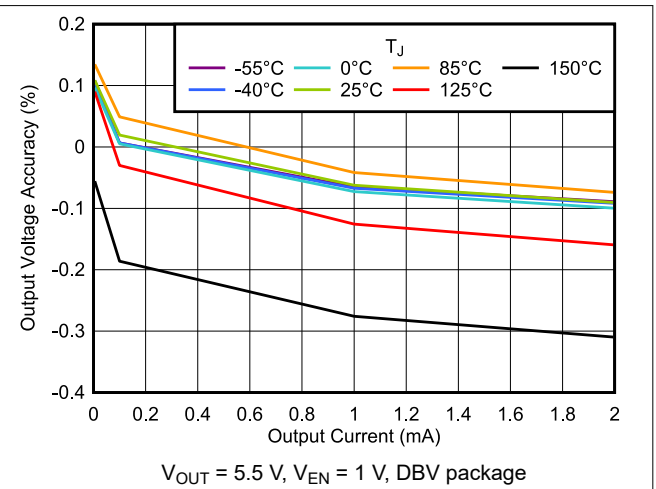
Figure 6-20. Output Voltage Accuracy vs I_{OUT}
