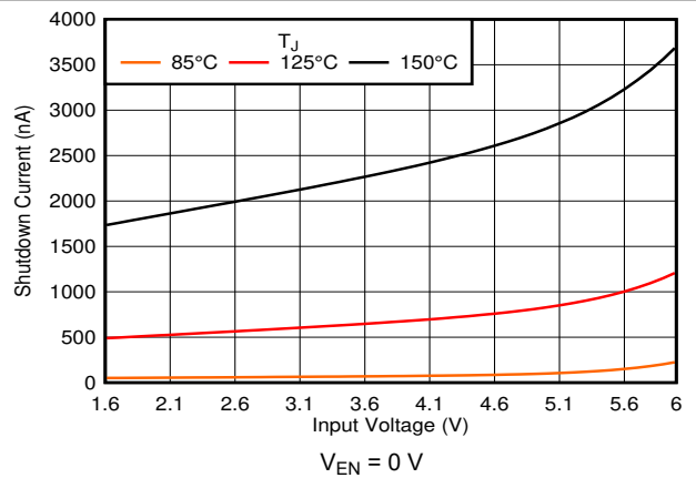
Figure 6-42. Shutdown Current vs V_{IN}
