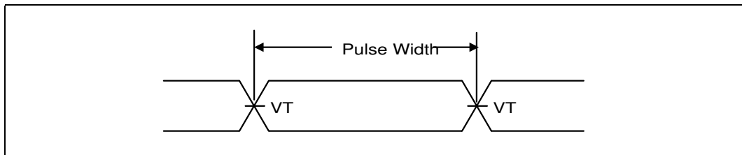
Figure 8-15. Pulse Width
