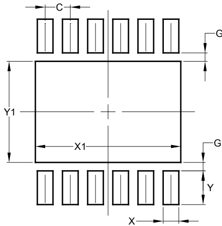
W-DFN3030-12 (Type US)
