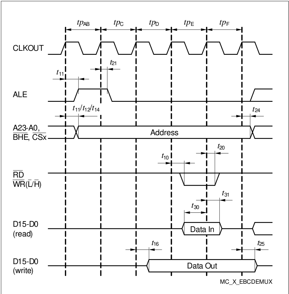
Figure 26 Demultiplexed Bus Cycle
