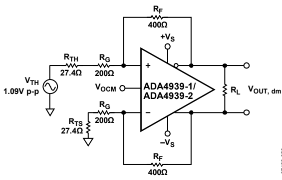
Figure 49. Thevenin Equivalent and Matched Gain Resistors
