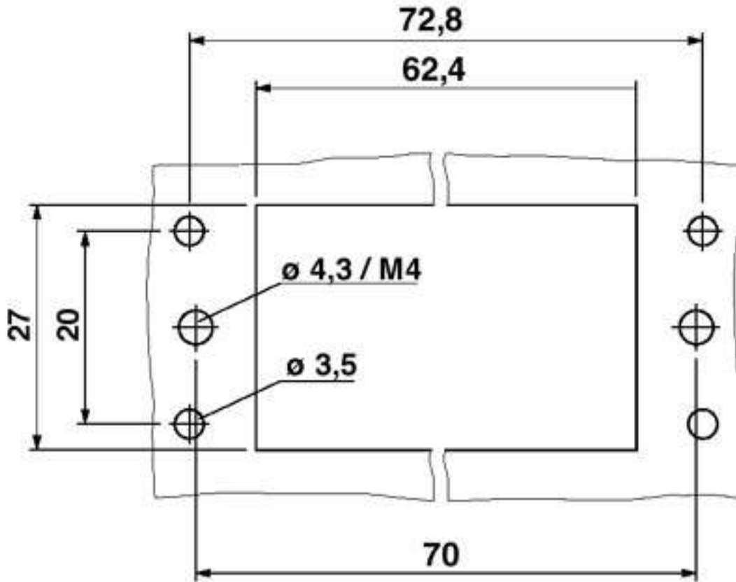
Panel cutout
