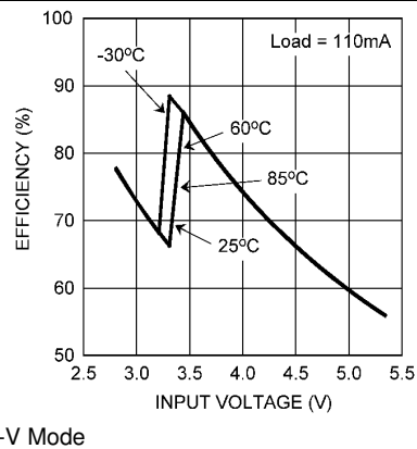
Figure 23. Efficiency vs. Input Voltage
