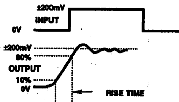
FIGURE 1. TRANSIENT RESPONSE
