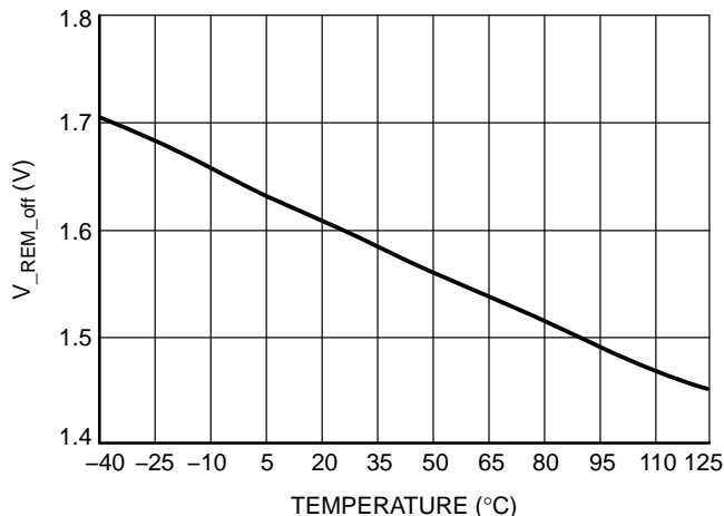
Figure 24. Off-mode Turn-on Threshold, V_{REM\_off} , A/B Version
