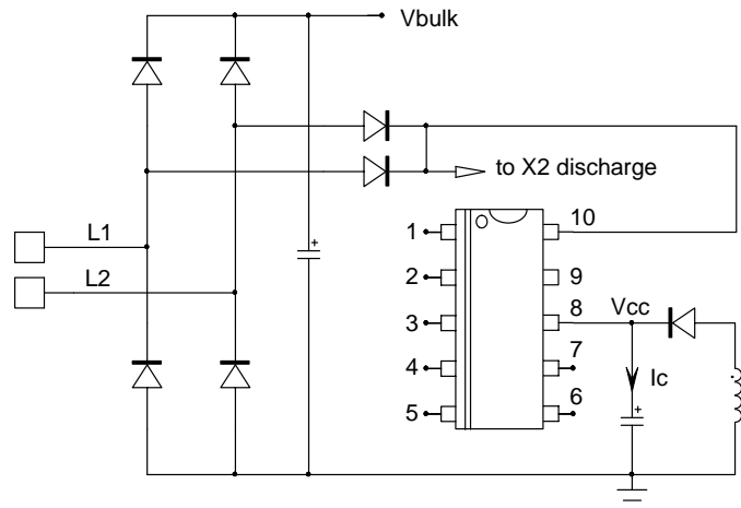
Figure 64. The startup resistor can be connected to the input mains for further power dissipation reduction
