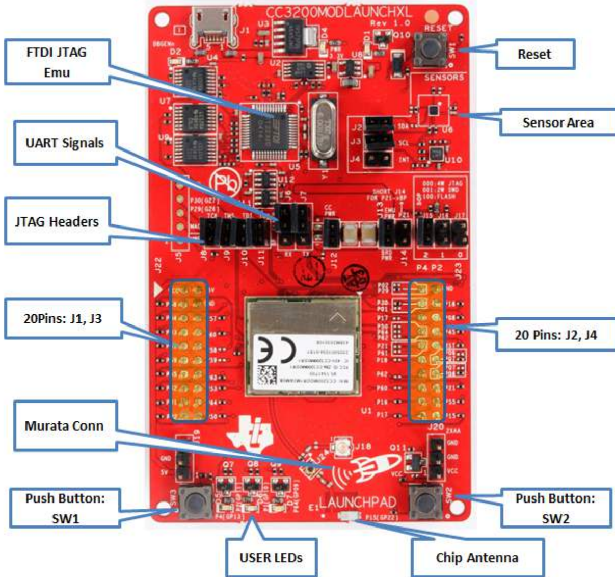
Figure 1. CC3200MOD LaunchPad EVM Overview
