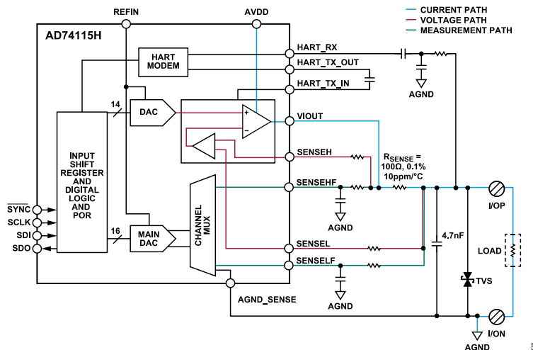
Figure 37. Current Input, Loop Powered Mode Configuration
