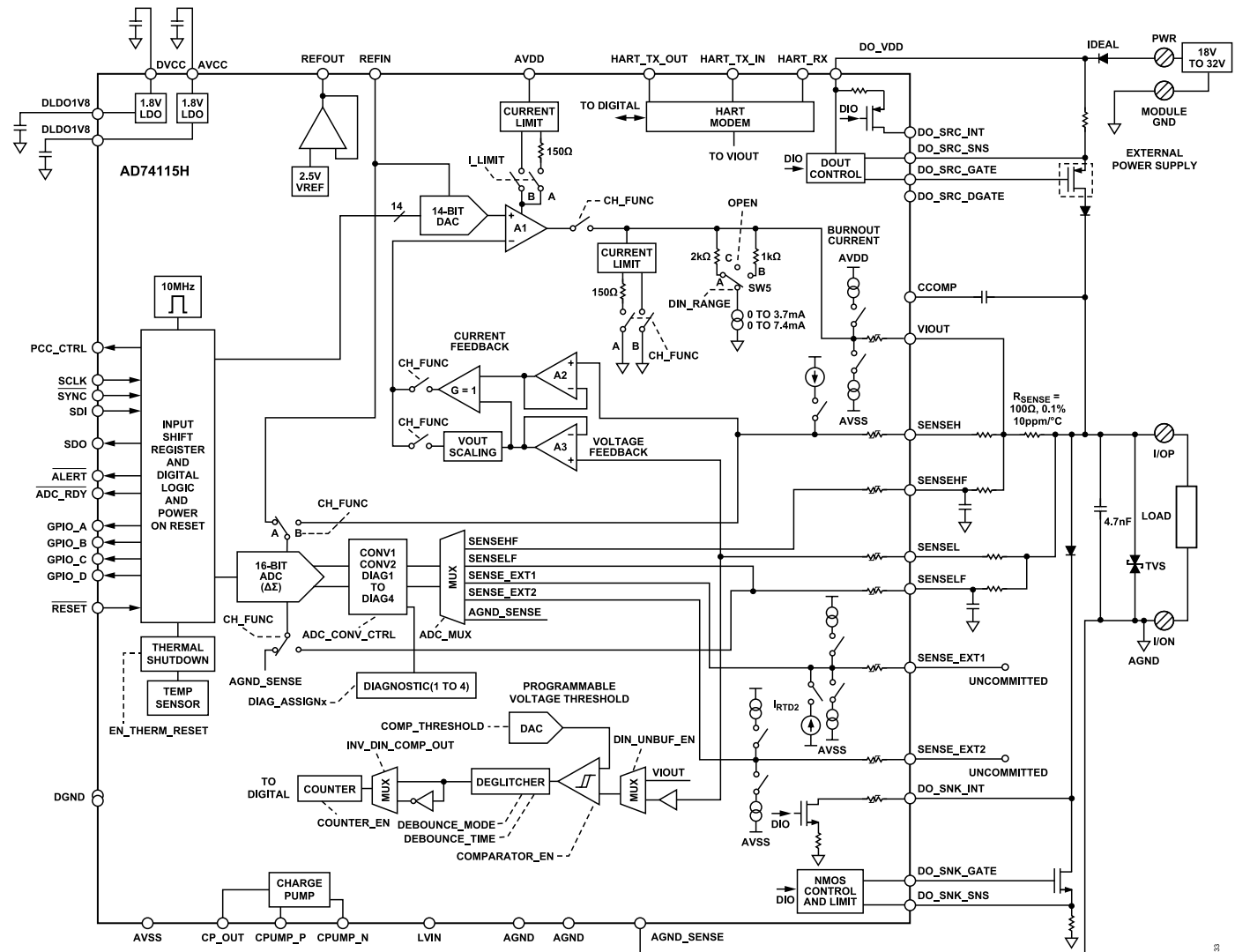
Figure 32. Detailed Functional Block Diagram
