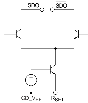
Fig. 10 \overline{\text{SDO}}/\overline{\text{SDO}} Output
