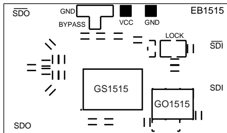
Fig. 24 Component Placement
