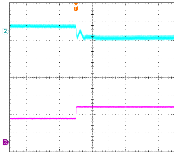
Figure 6: Transient Response
