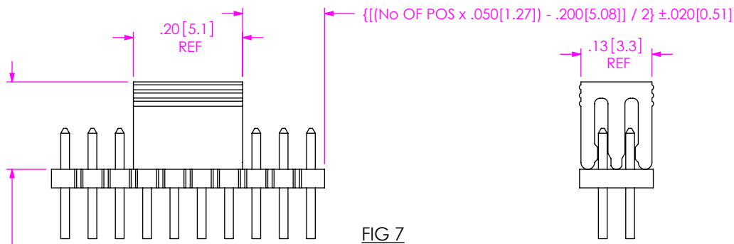
FIG 7 -D-P OPTION FTS-110-02-XX-D-P SHOWN (DIFFERENT AS SHOWN, OTHERWISE SAME AS FIG 1) "B" REF (SEE TABLE 3, SHT 2)
