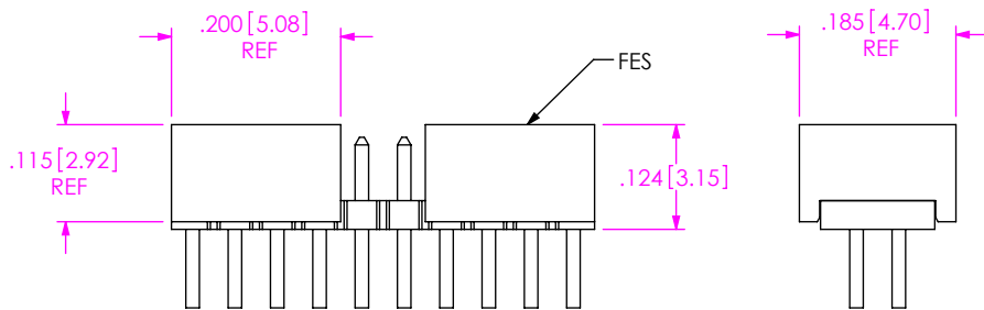
FIG 6 -D-S OPTION (SEE NOTES 6 & 7) FTS-106-02-XX-D-S SHOWN (DIFFERENT AS SHOWN, OTHERWISE SAME AS FIG 1) NOTE: 4 POSITIONS MUST BE ADDED TO PART CALLOUT TO ACHIEVE DIMS (NOT AVAILABLE WITH -A OPTION; ORDER -SA FOR ALIGNMENT PIN WITH SHROUD)
