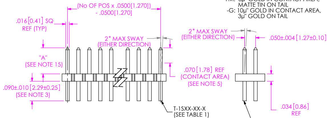
FIG 1 FTS-1XX-01-XX-D SHOWN
