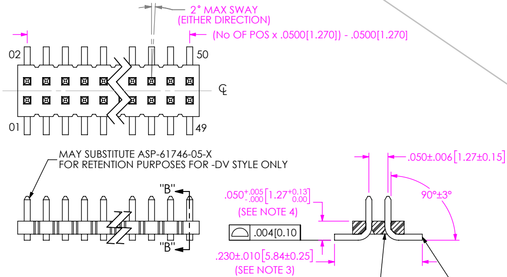
FIG 2 FTS-1XX-03-XX-DV SHOWN
