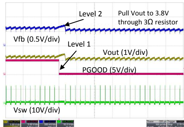
Figure 22. Over-Voltage Protection Level 1 and Level 2
