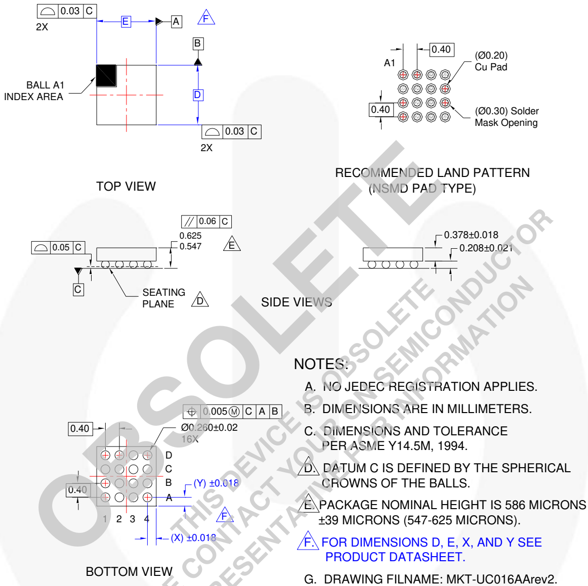
Figure 16. Wafer-Level Chip-Scale Package (WLCS)
